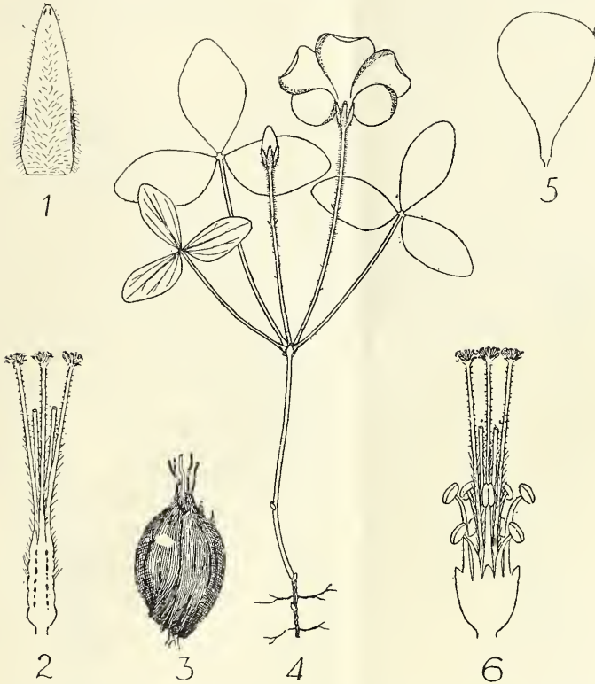
FIG. 4. Oxalis rhomboidea , Salter. 1. Sepal \times 6 . 2. Gynaecium \times 6 . 3. Bulb, natural size. 4. Plant, natural size. 5. Petal \times 1\frac{1}{2} . 6. Androecium \times 6 . (Salter 930.) Del. T. M. Salter.
